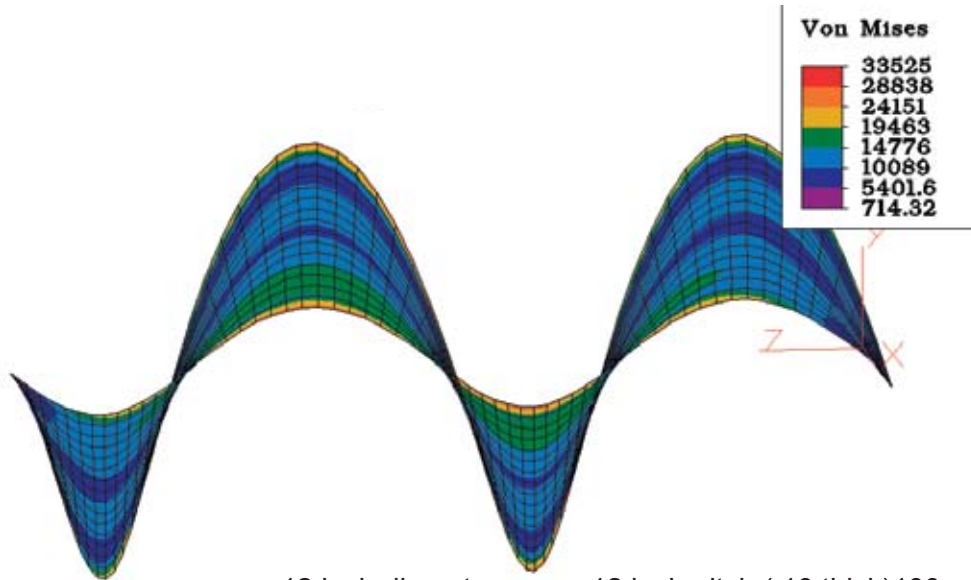
12 inch diameter screw 12 inch pitch (.10 thick)100 psi
